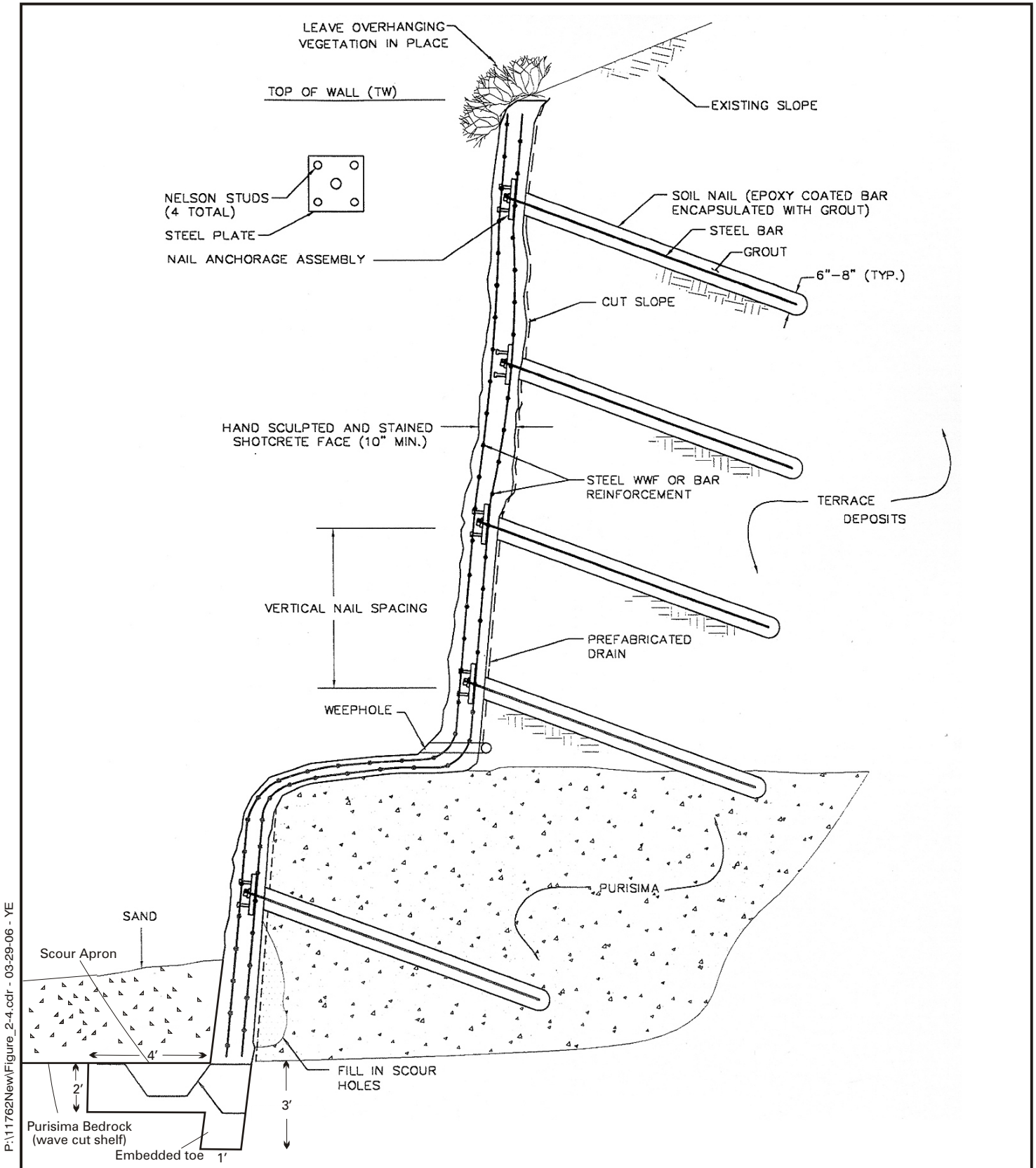
Typical soil nail construction, as proposed for alternatives 1, 2, and 3.
